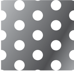
3/16" Dia 3/8" Ctrs 23% Open Area
