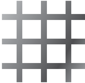
3/8" Sq 1/2" Ctrs 56% Open Area
