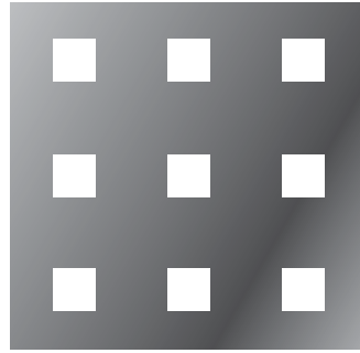
.200" Sq 1/2" Ctrs 16% Open Area
