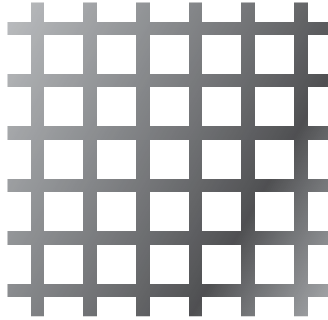
.200" Sq 1/4" Ctrs 64% Open Area
