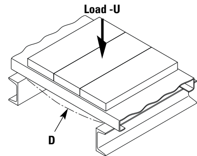
Figure 1c - Uniform Load
