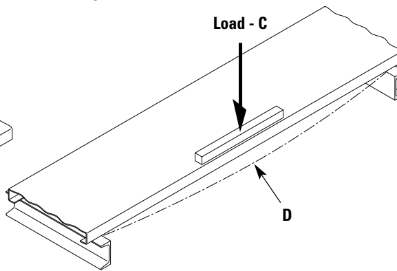
Figure 2b - Concentrated Load
